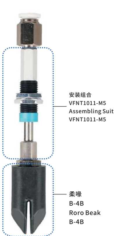
三尖外撑抓取珠宝 3 Pieces Application: Gripping jewelry by external bracing
